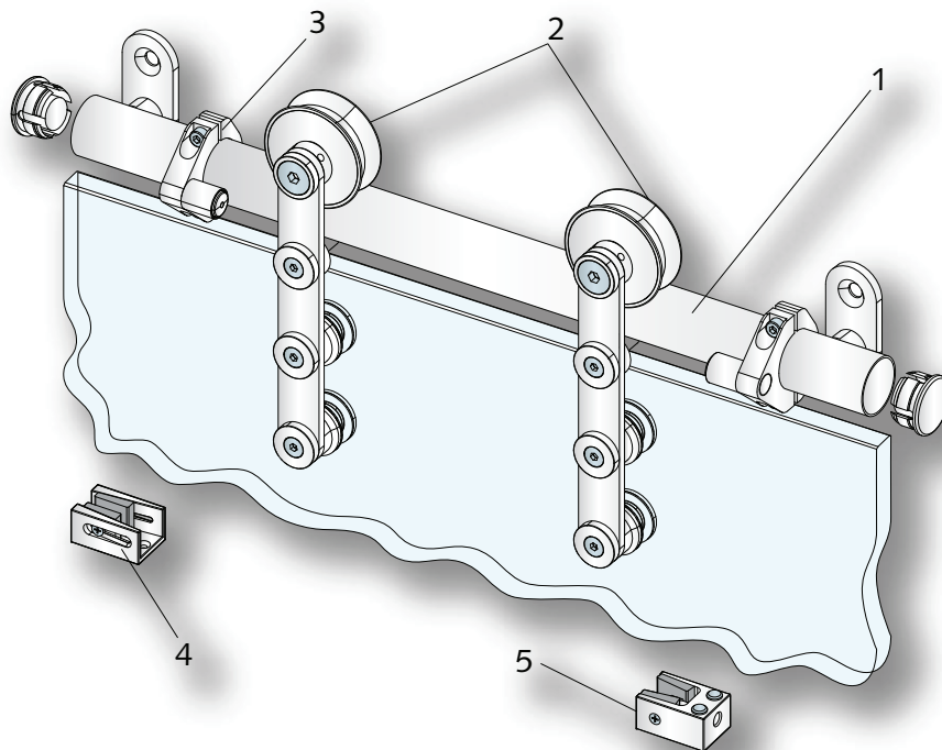
Components: 1. track with wall fixing, 2. carriers, 3. endstops, 4. floor guide, 5. floor stop
