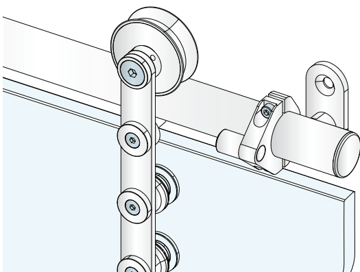
The holders allow a fast and secure wall installation of the track (track with wall fixing).
