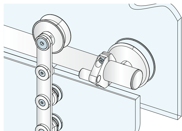
The clamping surfaces optimally disperse the pressure to the glass (track with glass fixing).
